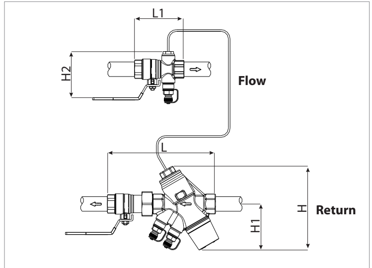
Frese PV System - Valve combination, capillary tube, isolation ball valve at the supply- and return line.
